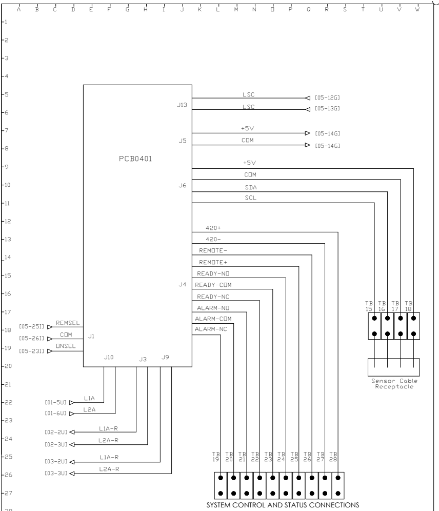
SYSTEM CONTROL AND STATUS CONNECTIONS - TECHNICAL INFORMATION
