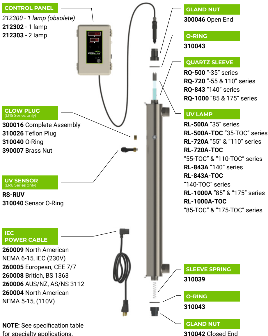
Figure 1. RAINIER System Components
