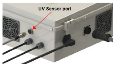
Figure 7. Sensor Connection
