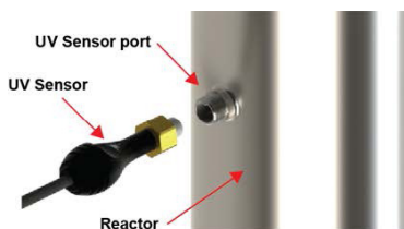
Figure 6. UV Sensor Installation
