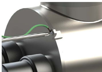
Figure 10. Ground Screw Connection
