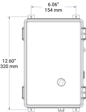
Figure 2. 1-Lamp Systems
