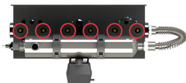
Figure 8. Pressure Gauge Ports
