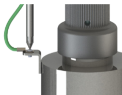
Figure 13. Ground Screw Connection
